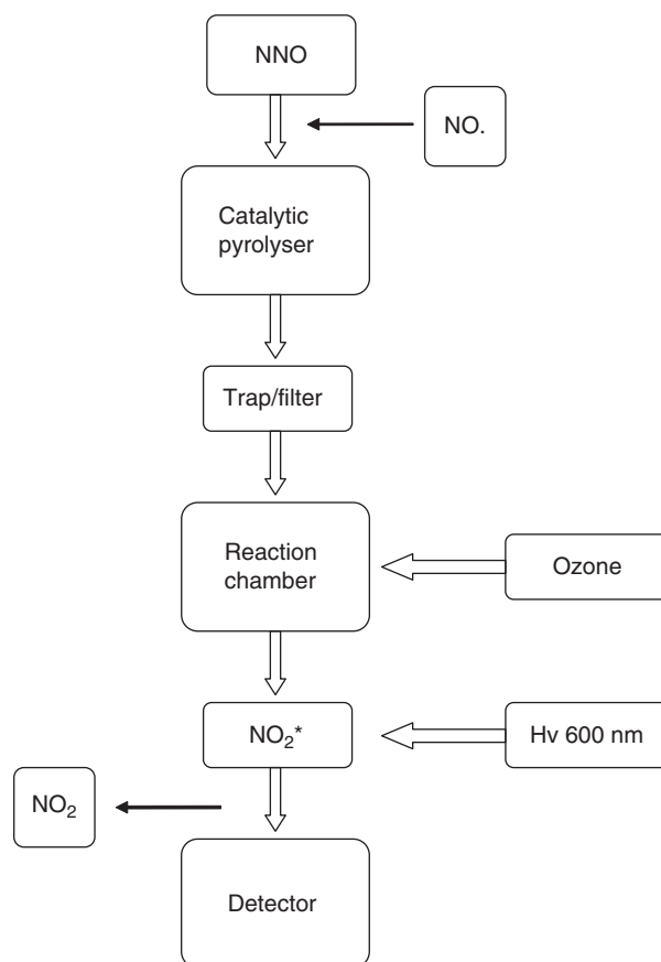
Figure 4 Schematic representation of the operation of nitrogen chemiluminescence detector.
