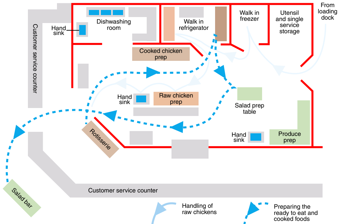
Figure 4 Physical facility layout.
